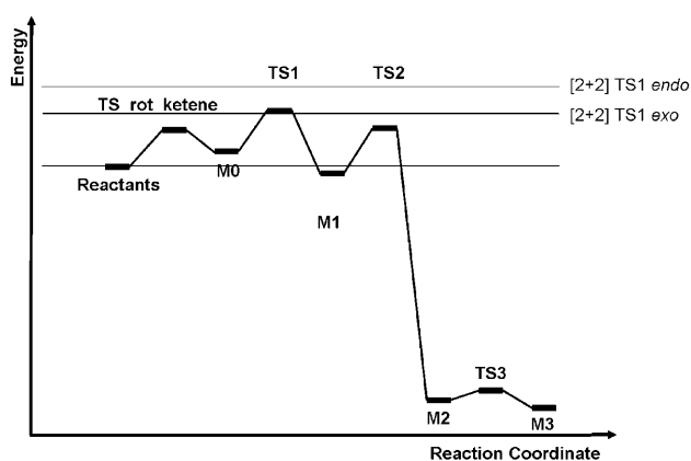
Figure 5. Energy profile for the 1E + 2A [4+2] reaction.
