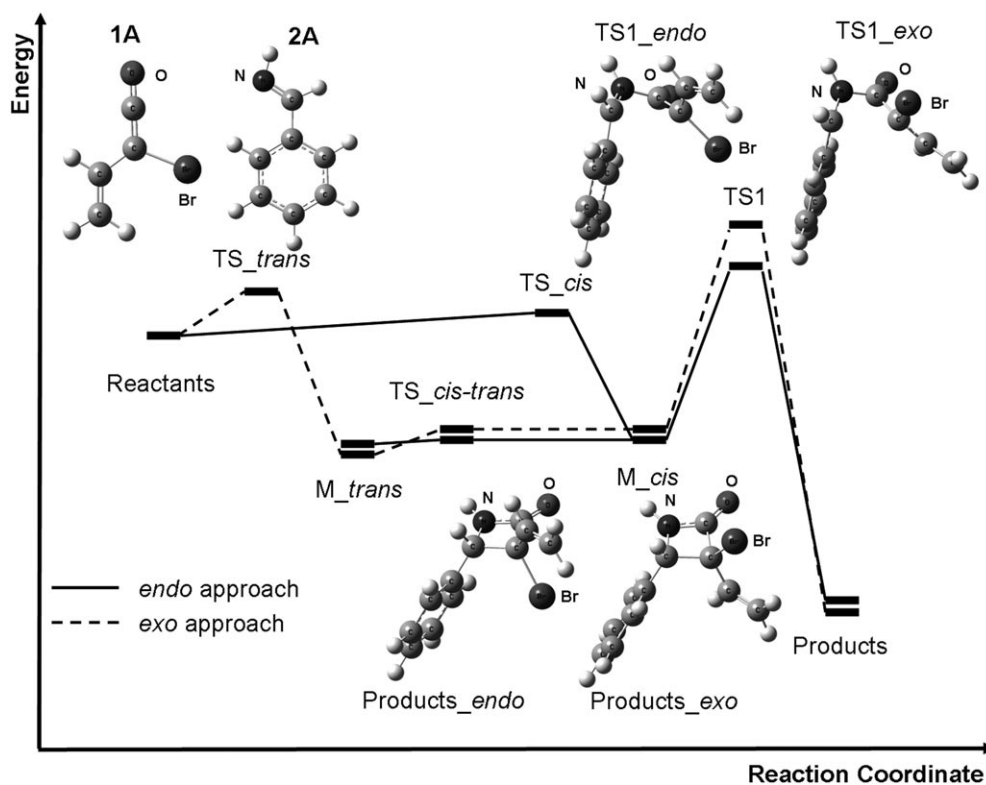
Figure 3. Energy profile for the 1A + 2A [2+2] reaction.
