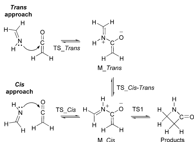
Scheme 7. Possible paths for the reaction between ketene and imine.
