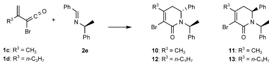
Scheme 5. Reaction of 1c and 1d with the chiral Schiff base 2e .
