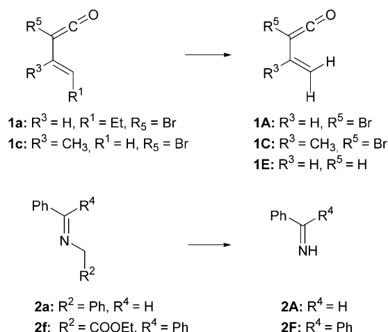
Scheme 8. Model systems ( 1A , 1C , 1E and 2A , 2F ) used in the computational study.
