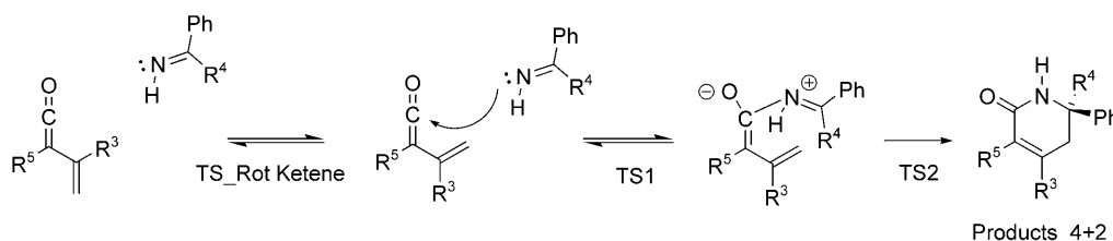
Scheme 10. General scheme for the [4+2] pathway.
