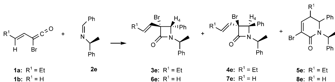
Scheme 3. Reaction of 1a and 1b with imine 2e .
