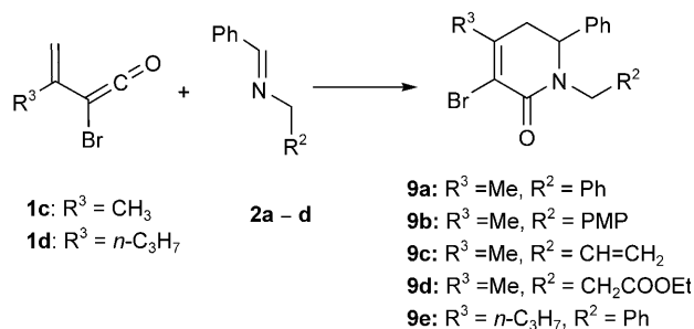
Scheme 4. Reaction of \beta -substituted- \alpha -bromo vinylketenes 1c–d with imines 2a–d .
