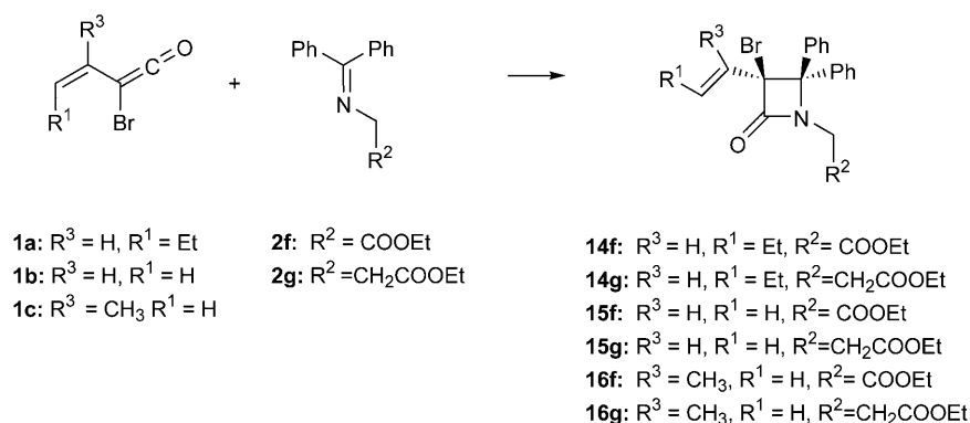
Scheme 6. Reaction of \alpha -bromo vinylketenes with ketimines 2f and 2g .
