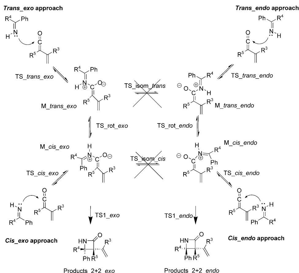
Scheme 9. General scheme for all possible [2+2] pathways.
