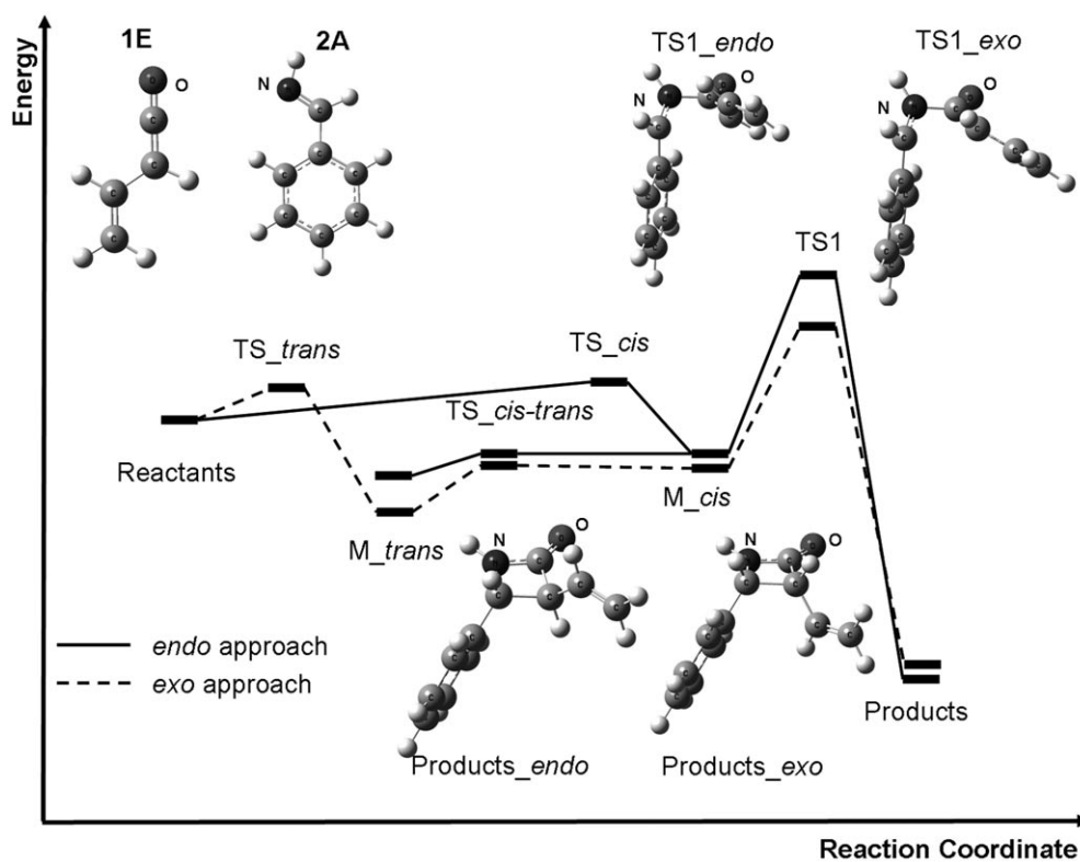
Figure 2. Energy profile for the 1E + 2A [2+2] reaction.
