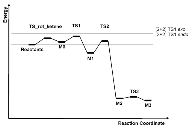
Figure 7. Energy profile for the 1C + 2A [4+2] reaction.
