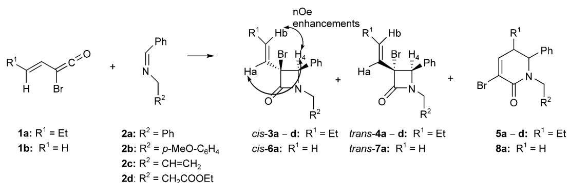
Scheme 2. Reaction of 1a and 1b with imines 2a–d .
