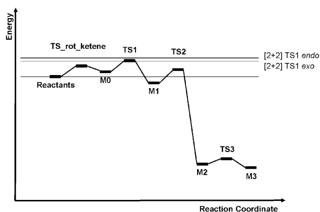
Figure 8. Energy profile for the 1C + 2F [4+2] reaction.
