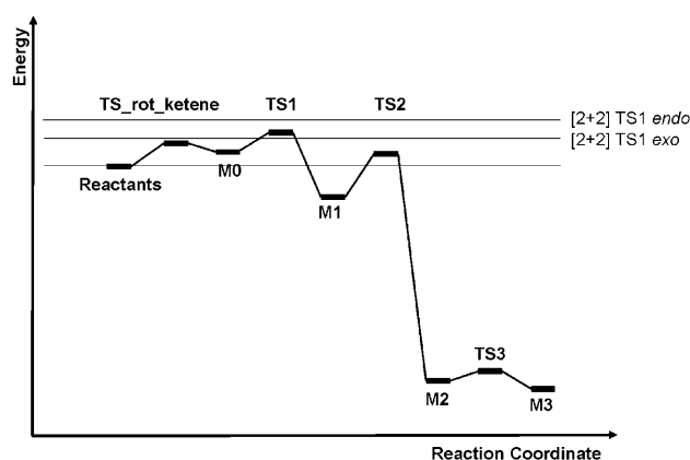
Figure 6. Energy profile for the 1A + 2A [4+2] reaction.
