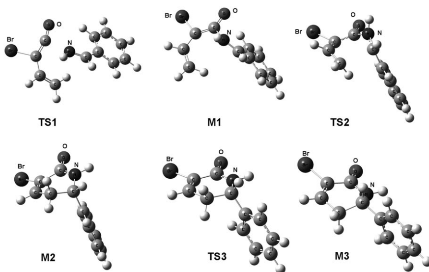
Figure 4. Structures of the various critical points located for the for 1E+2A [4+2] reaction.
