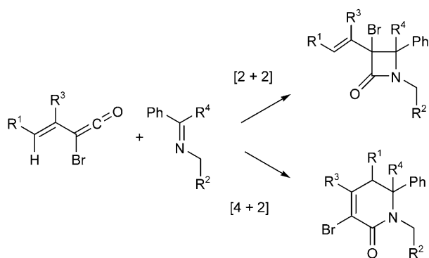
Scheme 1. Synthesis of 3-bromo-3-alkenylazetidin-2-ones and 3-bromo-4-alkyl-5,6-dihydropyridin-2-ones.
